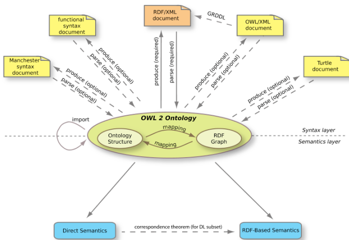
Fig. 1. The structure of OWL2
